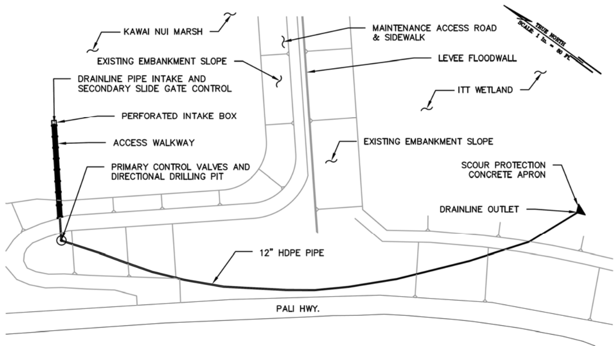
Figure 3. Alternative A3, directional drilling around end of levee within State DOT-highway right-of-way.
